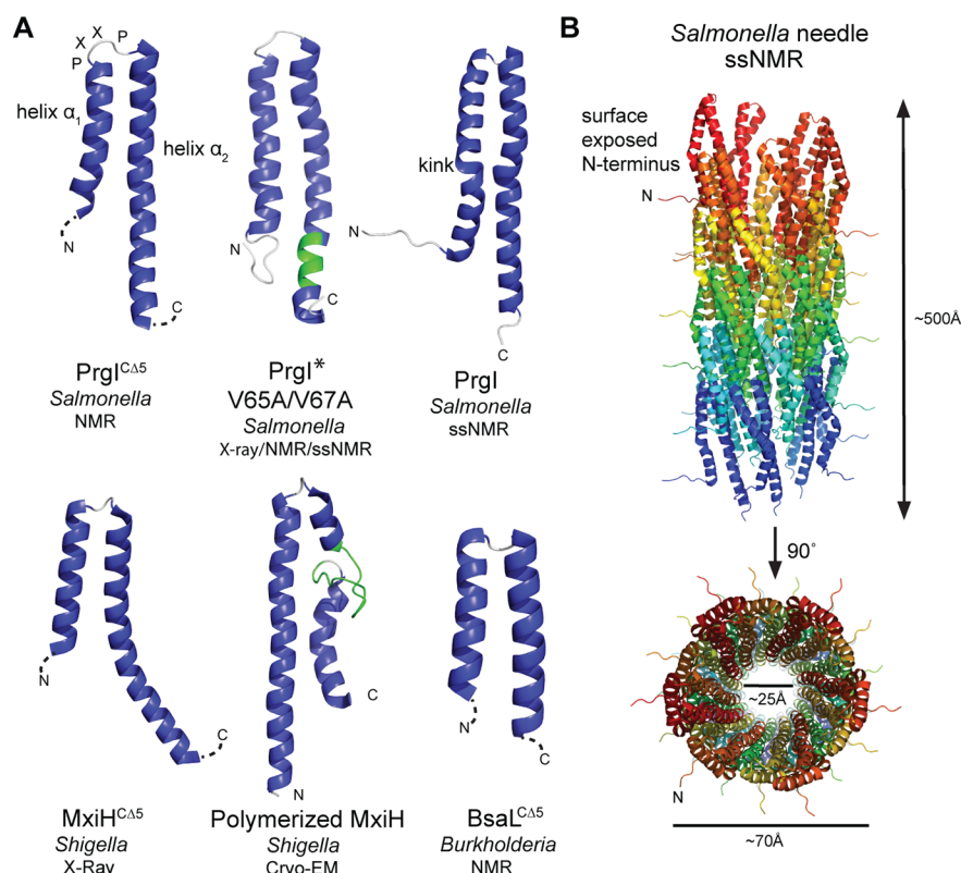
Figure 3. (A) Structures of needle protomers Salmonella PrgI CA5 (CA5, deletion of five C-terminal residues), 42 PrgI* (a functional V65A/V67A double mutant), 43 PrgI polymerized into needles, 48 Shigella MxiH CA5 , 40 MxiH polymerized into needles, 47 and Burkholderia BsaL CA5 . 41 Regions that adopted \beta -strands upon needle assembly are colored green. (B) Atomic model of the Salmonella needle derived by solid-state NMR showing that the N-terminus of PrgI faces the exterior. 48
